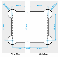
135° Glass to Glass for JHI302SQ
