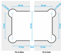
180° Glass to Glass for JHI303
