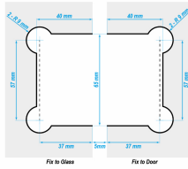
180° Glass to Glass for JHI303SQ
