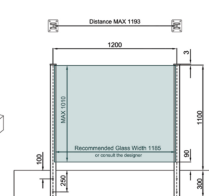
SIDE MOUNT - TOP CAP
