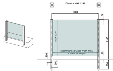
SIDE MOUNT - TOP CAP
