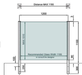
SIDE MOUNT - TOP CAP
