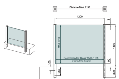
SIDE MOUNT - TOP CAP
