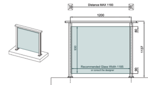
TOP MOUNT - HANDRAIL
