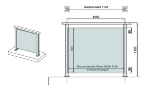
TOP MOUNT - HANDRAIL
