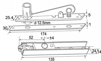
Adjustable top centre with \phi 12.5\text{mm} pin
